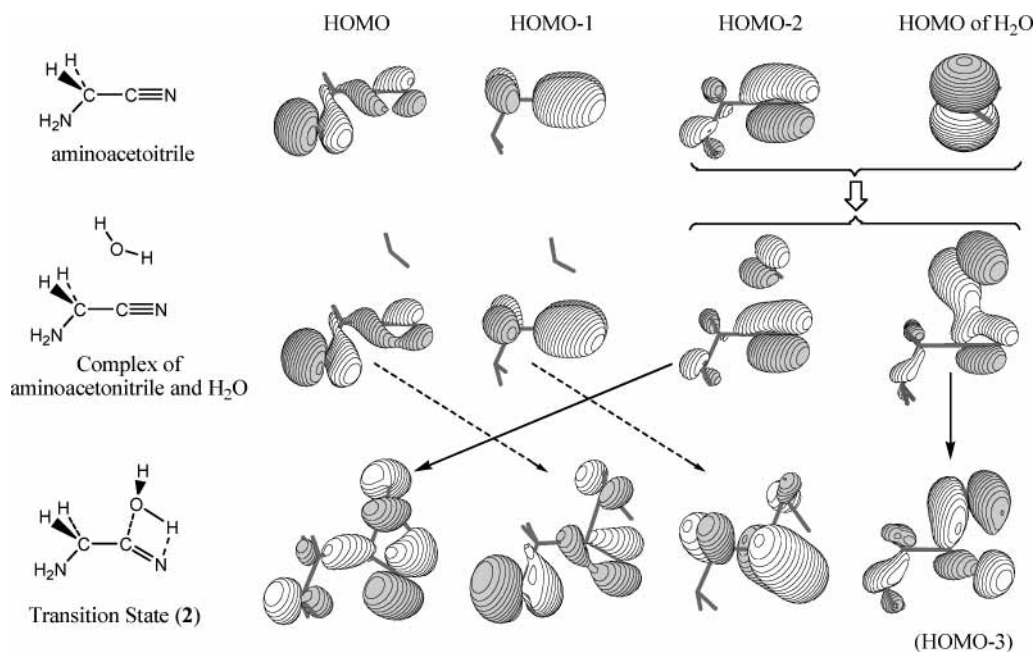
Figure 3. Shape of frontier orbitals (HOMO, HOMO-1, HOMO-2, and HOMO-3) of reactants (amino acetonitrile, complex of H 2 O and amino acetonitrile) and transition structure 2.
